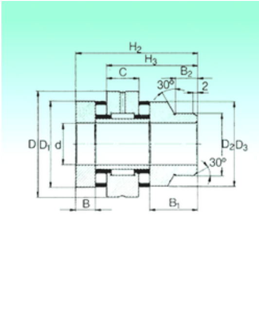
ZARN 3570 L TN Bearing 2D drawings and 3D CAD models
